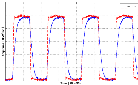
LVC MOS and EMI reduction Outputs, VDD = 2.5V
